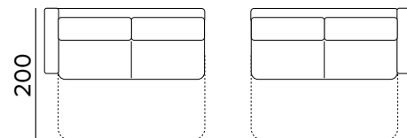
MATERASSO / MATELAS / MATTRESS CM 160x192 / H 13
