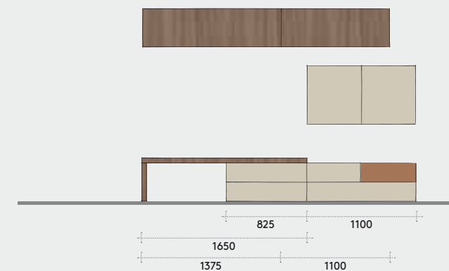
Comp. KV001A L 2750 H 2000 P 384/488
