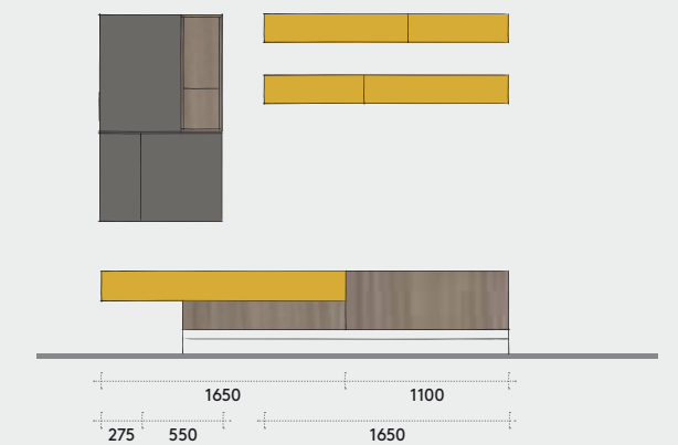
Comp. KV009B L 2750 H 2200 P 384/488
