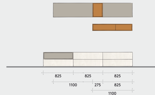
Comp. KV002A L 2475 H 1800 P 384/488
