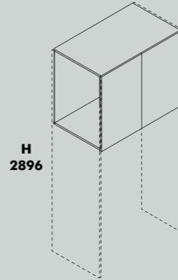
Moduli sopra porta L 1178 P. 494/498/592/596 W1178 Over door modules D.494/498/592/596
