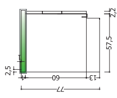
BASI H 73 BASE UNITS H 73
