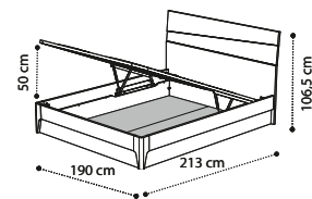
Letto 180 STORM c/contenitore Luna e rete 178x198 STORM bed 180 with Luna storage 178x198 Кровать 180 STORM с п/механизмом LUNA
