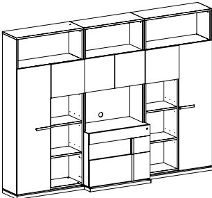
LIBRARY COMPOSITION 9 PJMN0808 inch W 114" D 21" H 84" cm L 290 P 52,7 H 213,4 Crts 9 kg 316 m 3 1,396
