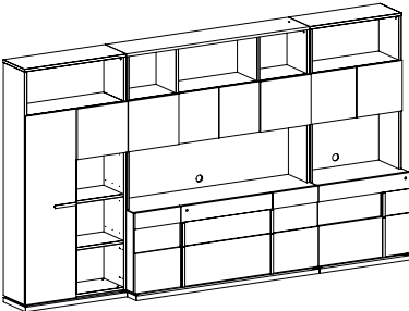
LIBRARY COMPOSITION 3 PJMN0802 inch W 146" D 21" H 84" cm L 369,6 P 52,7 H 213,4 Crts 11 kg 430 m 3 2,265
