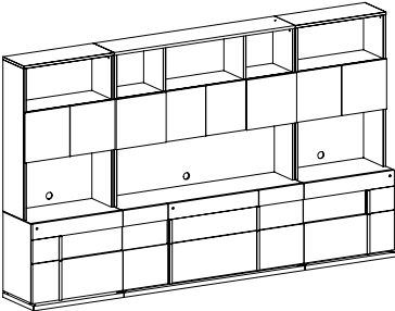
LIBRARY COMPOSITION 2 PJMN0801 inch W 142" D 21" H 84" cm L 359,6 P 52,7 H 213,4 Crts 11 kg 446 m 3 2,482
