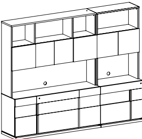
LIBRARY COMPOSITION 8 PJMN0807 inch W 106" D 21" H 84" cm L 269,6 P 52,7 H 213,4 Crts 8 kg 330 m 3 1,872
