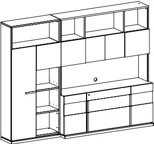
LIBRARY COMPOSITION 5 PJMN0804 inch W 110" D 21" H 84" cm L 279,6 P 52,7 H 213,4 Crts 8 kg 314 m 3 1,655
