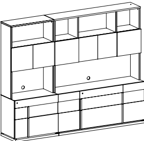
LIBRARY COMPOSITION 7 PJMN0806 inch W 106" D 21" H 84" cm L 269,6 P 52,7 H 213,4 Crts 8 kg 330 m 3 1,872
