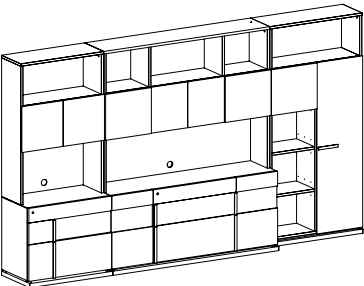
LIBRARY COMPOSITION 4 PJMN0803 inch W 146" D 21" H 84" cm L 369,6 P 52,7 H 213,4 Crts 11 kg 430 m 3 2,265
