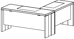
DESK COMPOSITION 2 PJMN0817 Desk + Return desk inch W 47" D 71" H 30" cm L 160 P 175 H 76 Crts 4 kg 93 m 3 0,315
