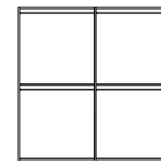
4/D SWINGING WARDROBE PJMA0012 With 4 doors, 2 shelves and 4 hanging rods inch W 90" D 24" H 94" cm L 228,7 P 61,5 H 239,1 Crts 8 kg 328 m 3 0,43
