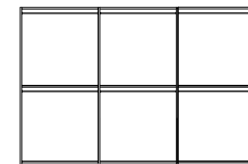
6/D SWINGING WARDROBE PJMA0014 With 6 doors, 3 shelves and 6 hanging rods inch W 135" D 24" H 94" cm L 341,8 P 61,5 H 239,1 Crts 10 kg 394 m 3 0,58
