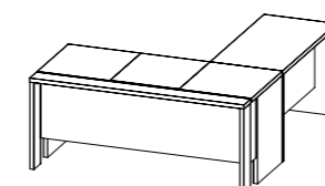
DESK COMPOSITION 1 PJMM0815 Desk + Return desk inch W 81" D 71" H 30" cm L 206 P 180 H 76 Crts 4 kg 124 m 3 0,42
