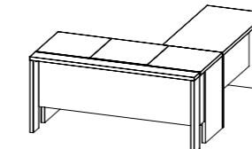
DESK COMPOSITION 2 PJMM0816 Desk + Return desk inch W 77" D 66" H 30" cm L 196,2 P 167 H 76 Crts 4 kg 114 m 3 0,38
