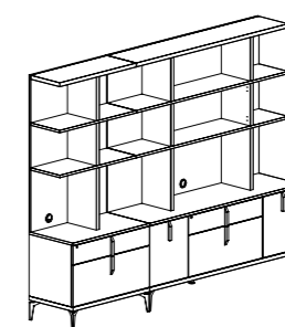
LIBRARY COMPOSITION 7 PJMM0806 inch W 106" D 20" H 84" cm L 270,2 P 52 H 212,2 Crts 7 kg 297 m 3 1,60
