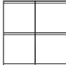
4/D SWINGING WARDROBE (wooden doors) PJCL0013 (with 2 central mirrors) PJCL0014 With 4 doors, 2 shelves and 4 hanging rods inch W 78" D 25" H 90" cm L 197,3 P 64,7 H 227,5 Crts 8 kg 221/243* m 3 0,61/0,61*
