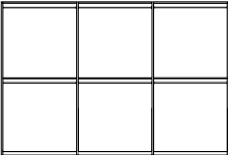
6/D SWINGING WARDROBE** (wooden doors) PJCL0017 (with 2 mirrors) PJCL0018 With 6 doors, 3 shelves and 6 hanging rods inch W 116" D 25" H 90" cm L 295 P 64,7 H 227,5 Crts 10 kg 319/341* m 3 0,79/0,79*
